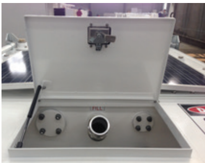
80 NB FILL POINT WITH CAMLOC AND CAP
